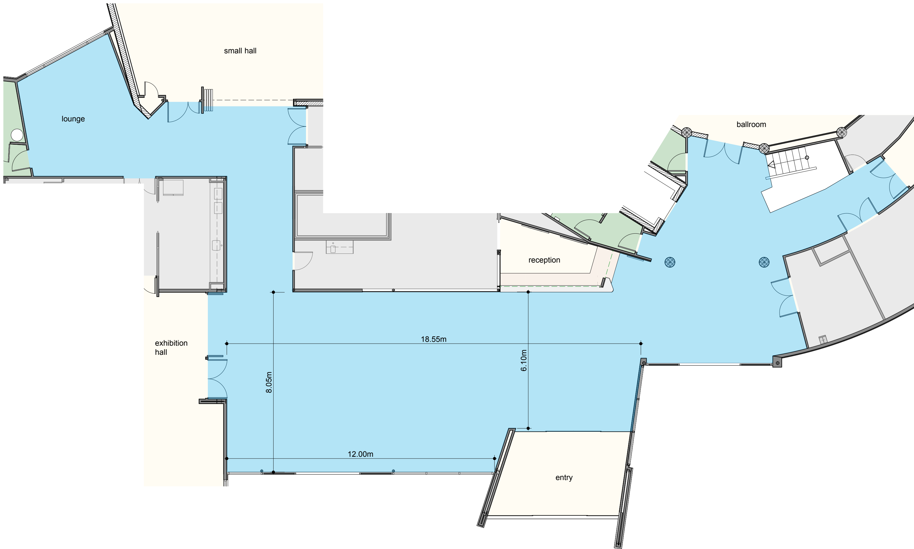
FOYER 275 sqm
